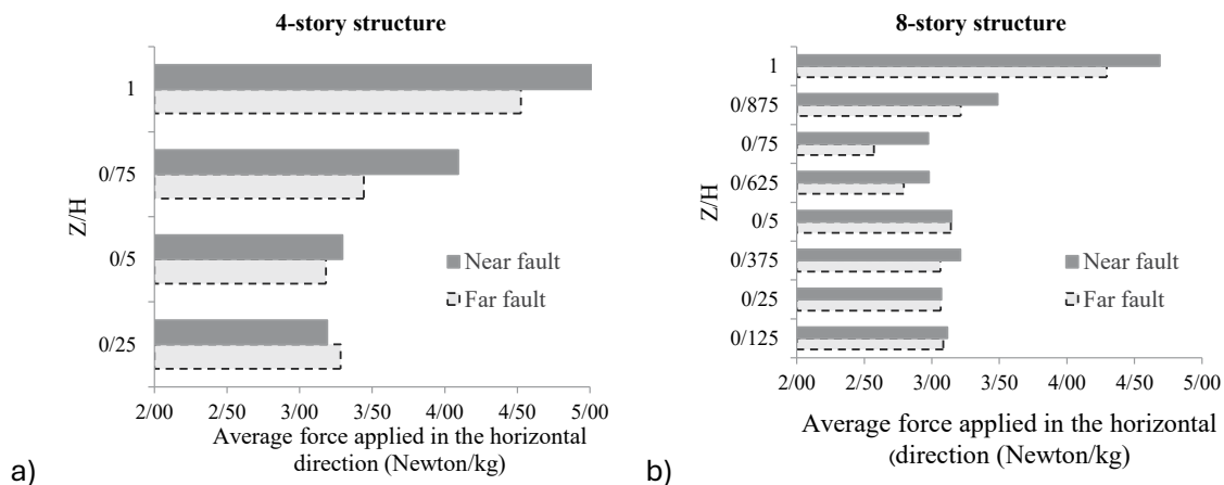
Figure 5. Average horizontal forces exerted on a unit-mass suspended ceiling under far-field and near-fault ground motion suites at various floor levels: (a) 4-story structure, (b) 8-story structure
