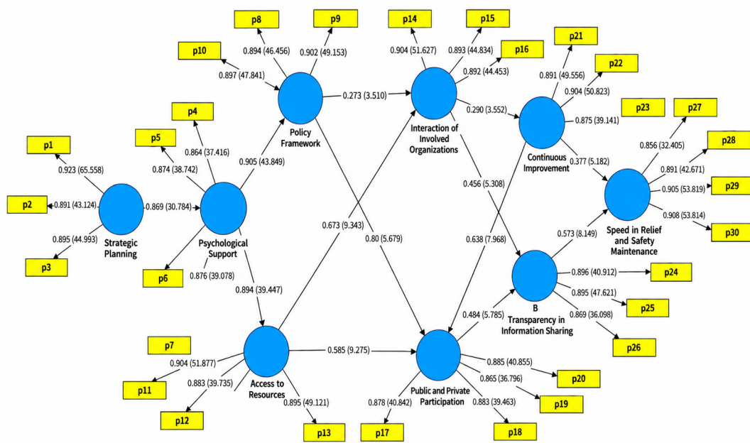
Figure 3. Conceptual research model with t statistics, path coefficients, and factor loadings
