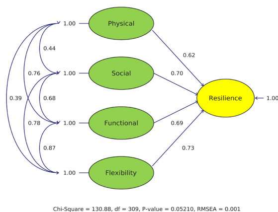
Figure 5. SEM: Pearson correlation coefficients and relationships among the indicators
