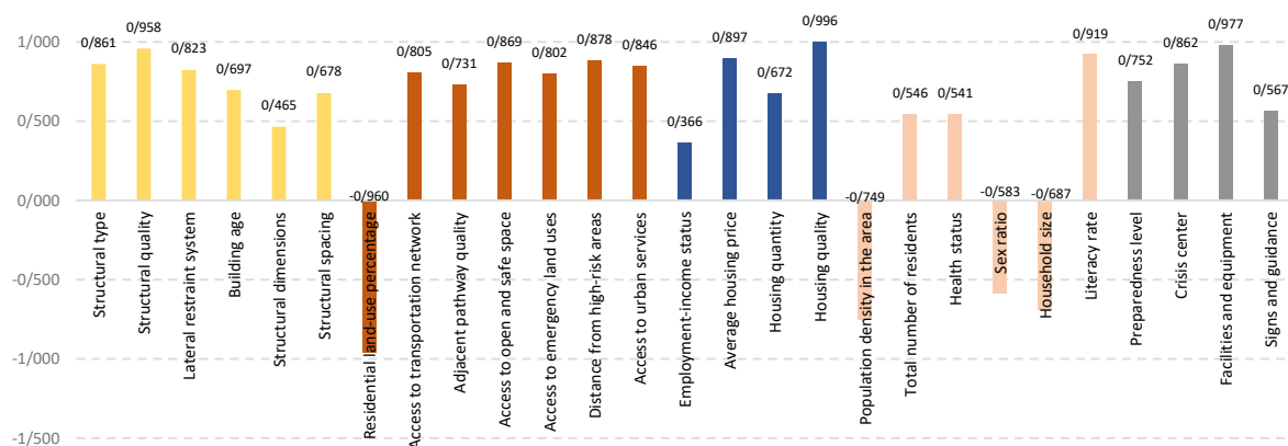
Figure 4. Factor loadings of the variables (based on the data presented in table 9)
