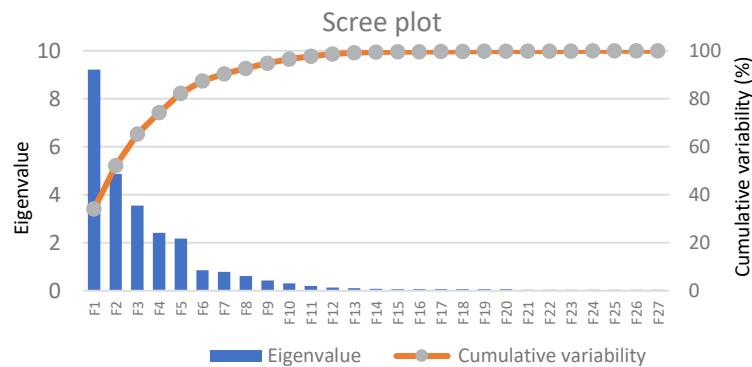
Figure 3. Scree plot of eigenvalues for extracted components (PCA method)
